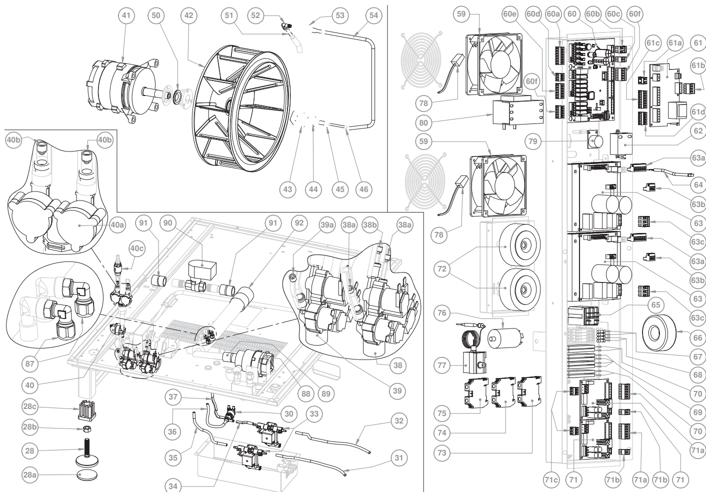
Exploded view 2/4
