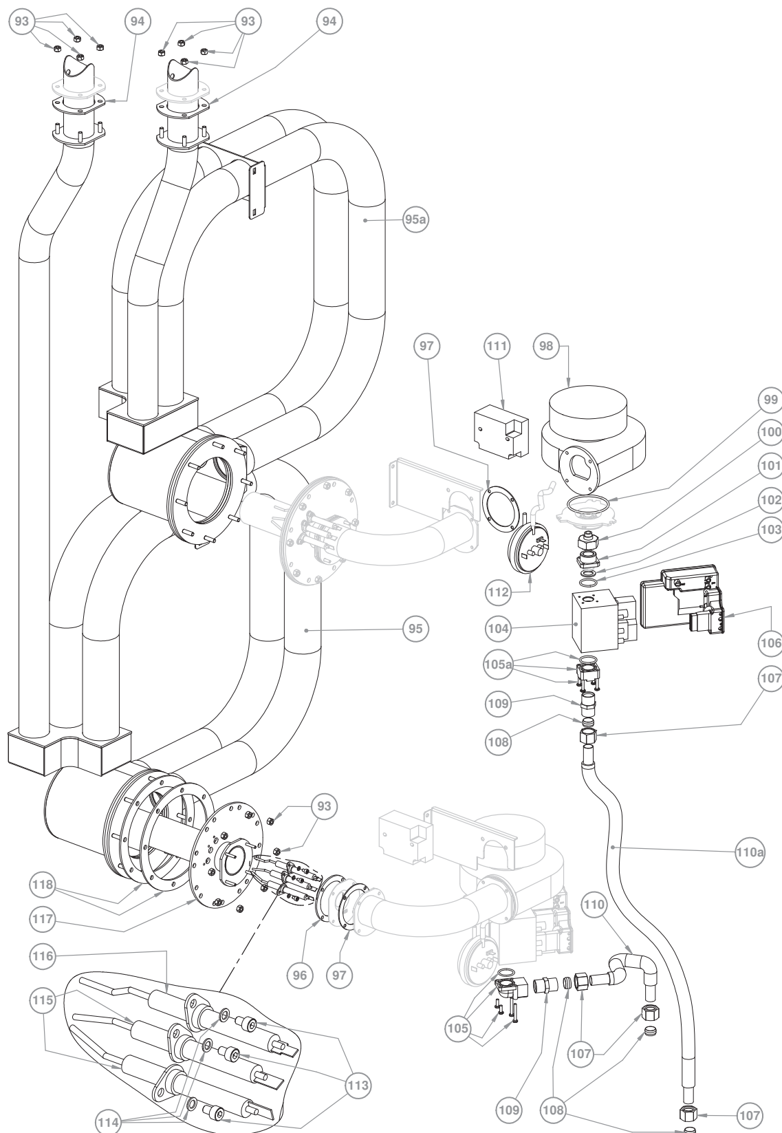
Exploded view 4/4
