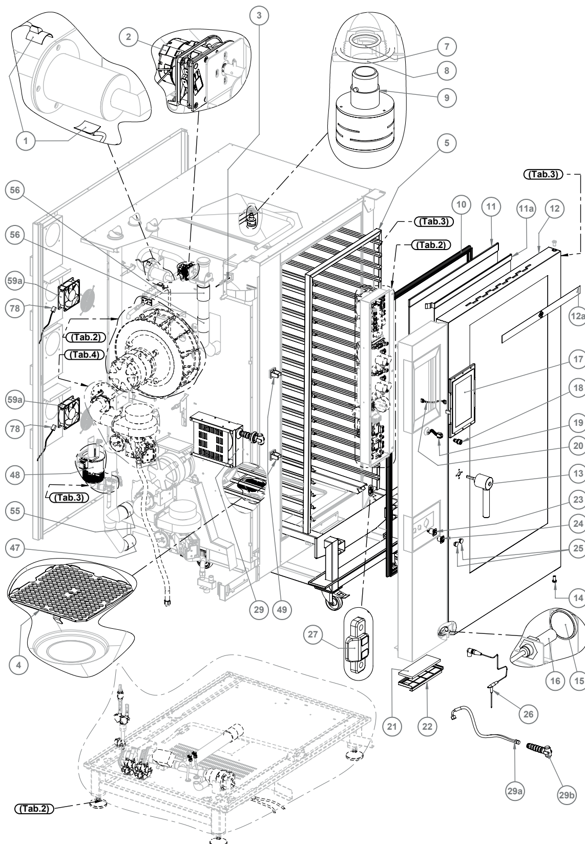
Exploded view 1/4
