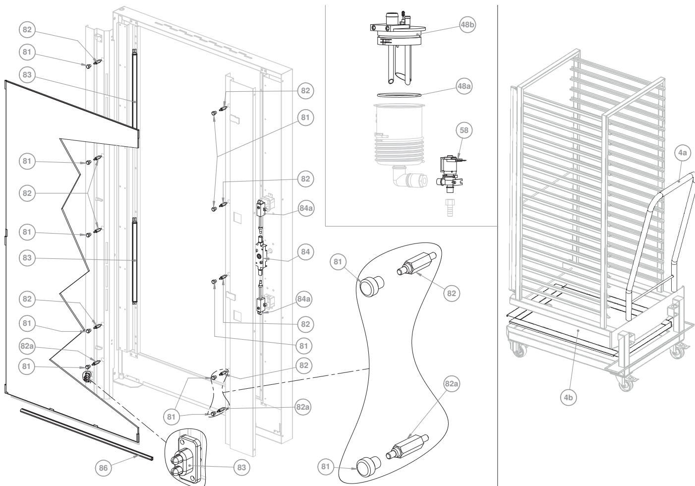
Exploded view 3/4
